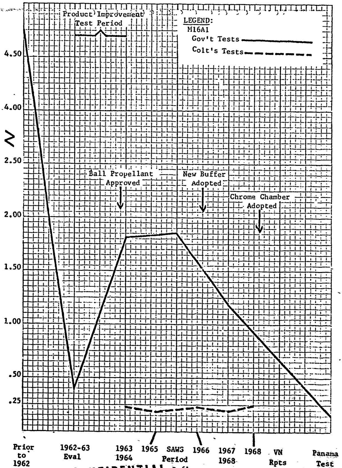
Figure II-9 — ALL OTHER M16 MALFUNCTIONS
